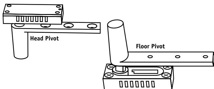
HA500 Single action pivot set
