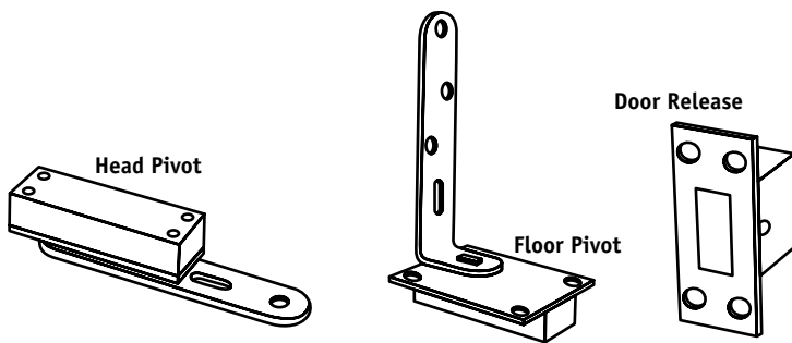
HA611 Double action pivot set. Mortise application in masonry floor.
