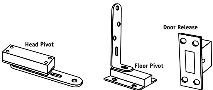
HA612 Double action pivot set. Surface application in masonry/wood floor.
